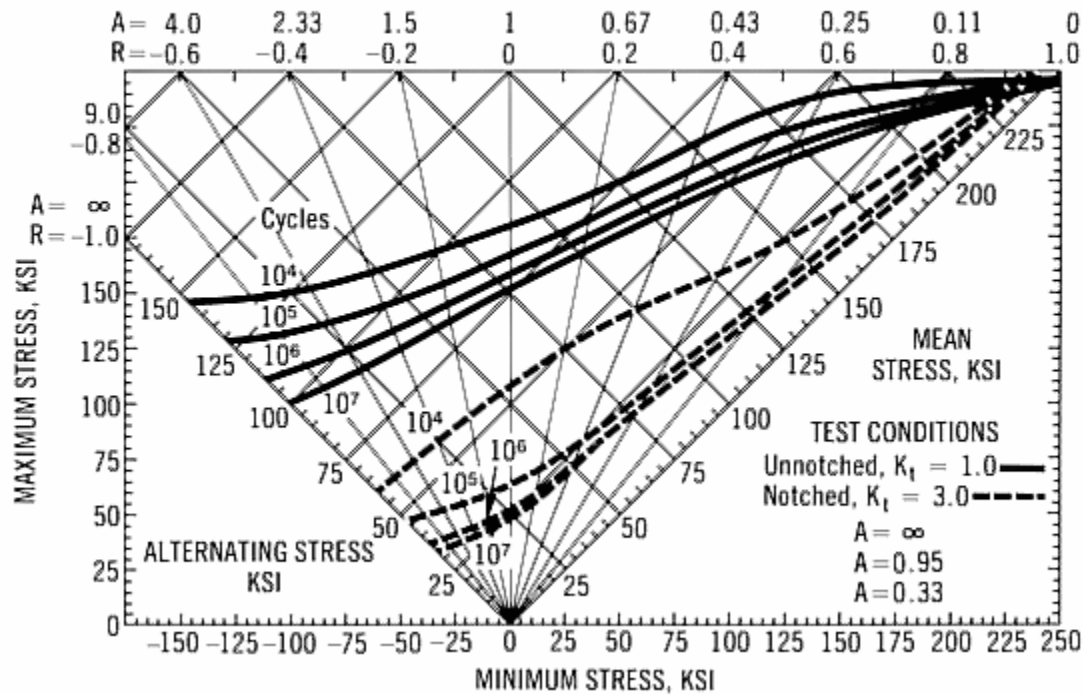
Typical Constant Life Fatigue Diagram for Custom 455 Stainless Bar in the H 950 Condition at Room Temperature (Axial tests using longitudinal specimens)
